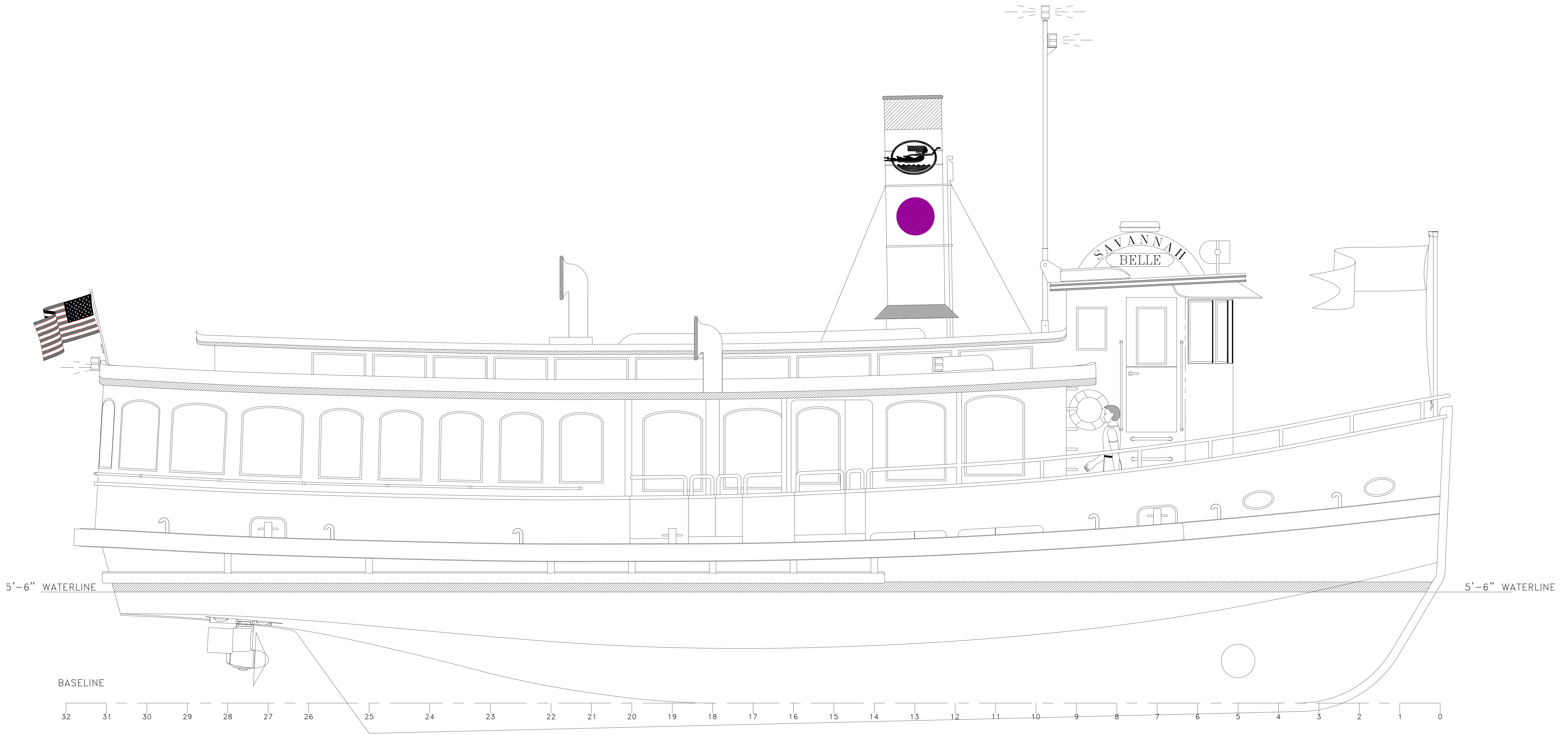
OUTBOARD PROFILE
