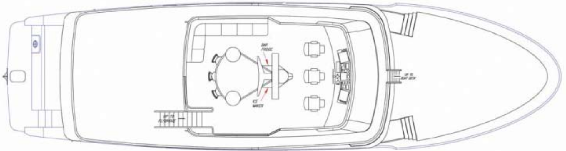
Custom Steel 82 Flybridge Deck
